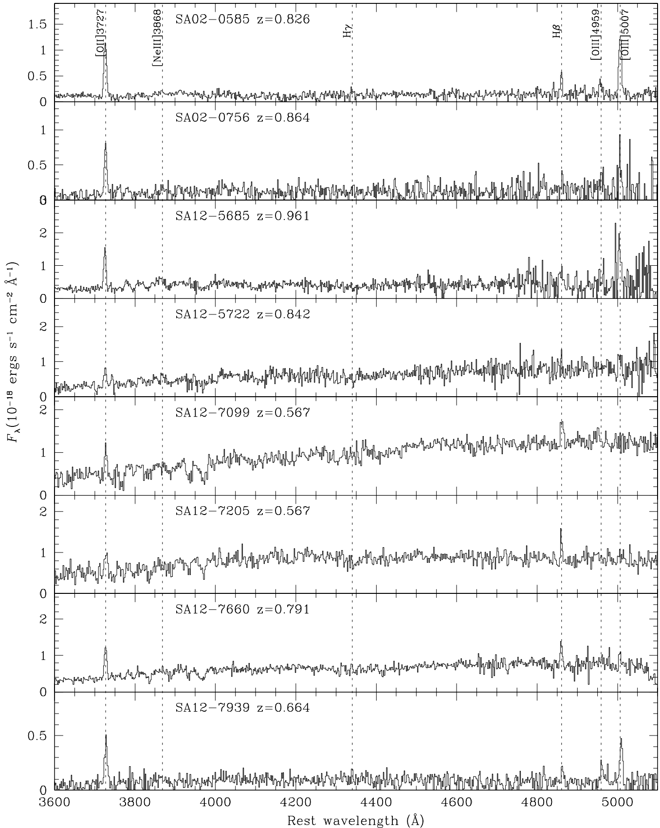
FIG. 2.— The sample of GDDS galaxies at 0.4 < z < 1 . Relevant emission lines are marked by the vertical dashed lines.
