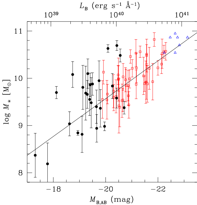
FIG. 8.— Stellar Mass and B absolute magnitude (or luminosity, upper horizontal axis) for the GDDS (filled circles) and CFRS (open squares) z < 1 galaxies. The open triangles are the z \sim 2.3 LBGs (Shapley et al. 2004) after correcting the stellar mass for BG03 IMF. The straight line marks a constant ratio of stellar mass to B luminosity, in solar units, of M_{*,\odot}/L_{B,\odot} = 0.3 .
