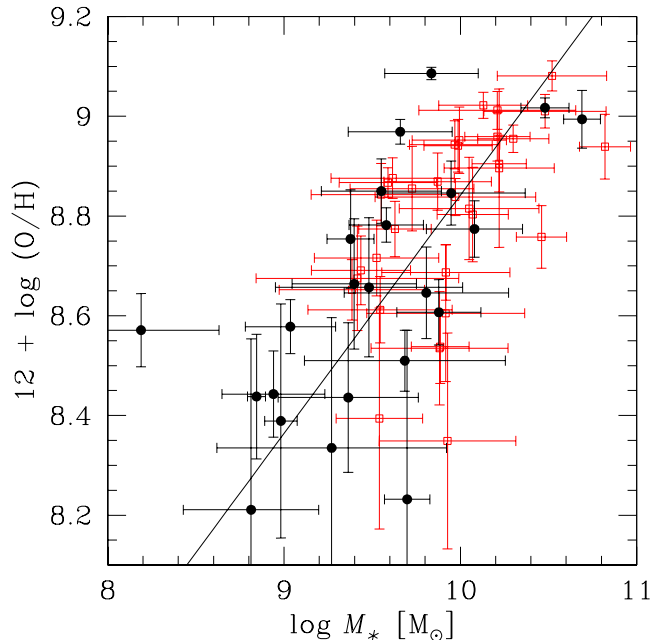
FIG. 12.— Metallicity as a function of stellar mass for GDSS (filled circles) and CFRS galaxies (open squares). Error bars include measurement errors but not possible systematic effects. The straight line is the linear bisector fit. The correlation is more than 6\sigma significant. The metallicity scale is as in Figure ??, and the mass scale spans three orders of magnitudes, as in the luminosity scale of the upper x -axis of Figure ?. This way it is possible to visually compare the point scatter in the two figures.
