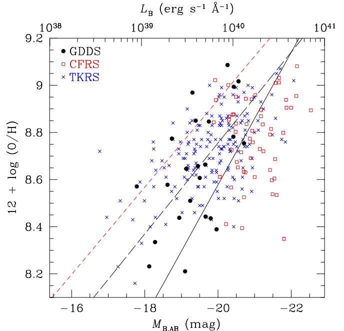
FIG. 11.— 12 + \log(\text{O}/\text{H}) as a function of B absolute magnitude M_{B,AB} (or luminosity, upper horizontal axis) for the GDSS (filled circles), CFRS (open squares) and TKRS (crosses; KK04). The linear bisector fits (see text) for GDSS+CFRS and TKRS are shown as solid and long-dashed lines, respectively. The short-dashed line is the luminosity-metallicity relation found for the SDSS sample at z \sim 0.1 (Tremonti et al. 2004).
