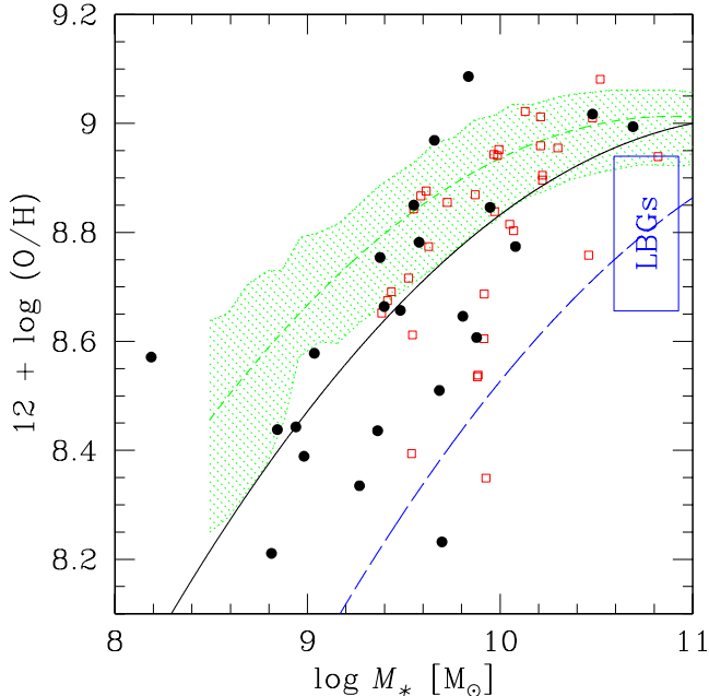
FIG. 13.— Metallicity as a function of stellar mass for GDDS (filled circles) and CFRS (open squares). The points are as in Figure ??, but error bars are omitted. The green short-dashed line and hatched area indicate the polynomial fit and \pm 1\sigma dispersion, respectively, derived for the SDSS z \sim 0.1 galaxies (T04). The blue rectangle is the region occupied by the LBGs at 2.1 < z < 2.4 (Shapley et al. 2004) after correcting from the N2 to the R_{23} calibrator. The black-solid and blue long-dashed lines are the SDSS polynomial shifted to the right to match the galaxy distributions at z \sim 0.7 and z \sim 2.3 , respectively.
