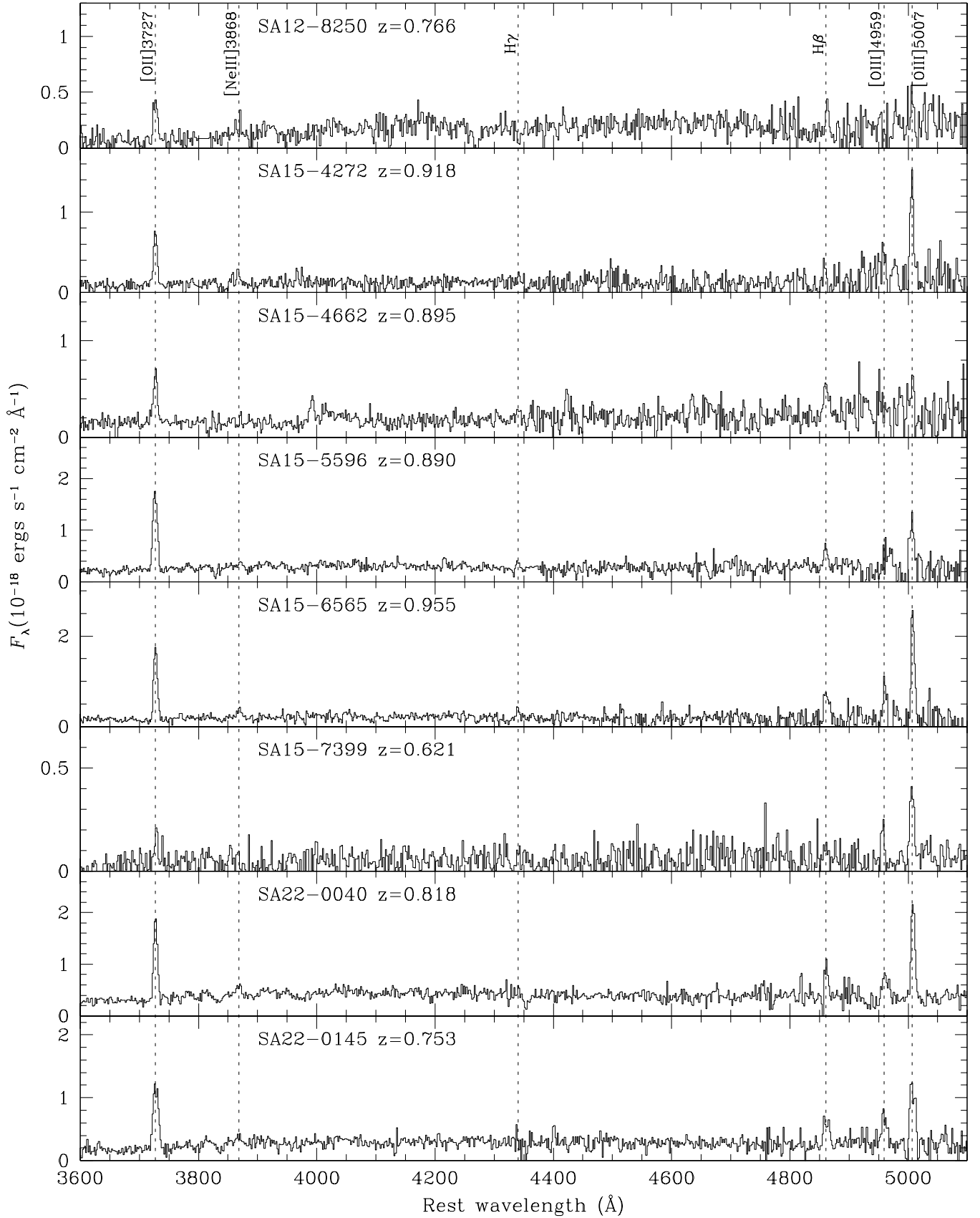
FIG. 3.— As in Figure ???. The spurious emission line at \lambda \sim 4000 \text{ \AA} in the spectrum of SA15-4662 is due to order overlap in the GMOS mask (see text).
