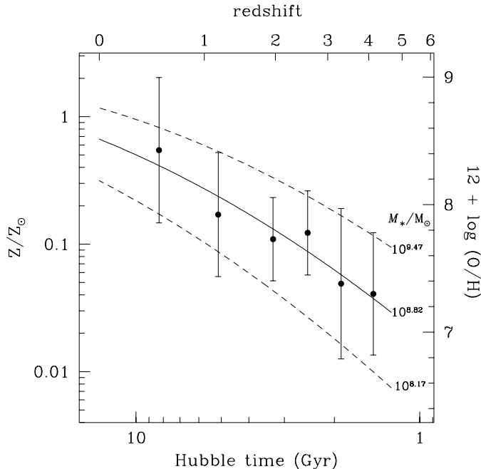
FIG. 17.— Comparison between mean metallicity in DLAs for different redshift bins (Savaglio 2001), and our empirical model of Eq. ???. The best fit gives a stellar mass for DLAs of 10^{8.82} M_{\odot} (solid line) with a dispersion of 0.65 dex (dashed lines). In this figure we made a correction of -0.3 dex to the model to account for a metallicity gradient in DLAs (Chen et al. 2005). The best-fit mass would be 0.3 dex higher if the R_{23} metallicity, used to calibrate the empirical model, is underestimated by a factor of 2 (Kennicutt et al. 2003).
