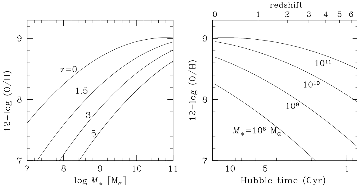
FIG. 15.— 12 + \log(O/H) as a function of stellar mass for constant redshifts ( left panel ), or as a function of Hubble time for constant stellar masses ( right panel ). These relations are obtained by extrapolating at all redshifts the z \sim 0.1 SDSS and our z \sim 0.7 M-Z relations. We emphasize that this empirical model is derived using the KK04 metallicity calibrator and BG03 IMF, and is different if other calibrators and IMFs are used.
