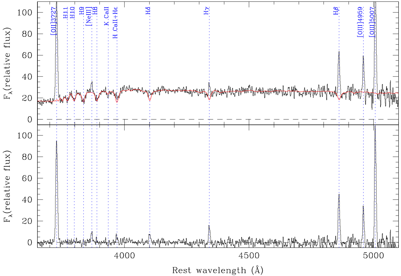
FIG. 7.— Composite spectrum of 26 0.4 < z < 1 GDDS galaxies. The dotted vertical lines mark the relevant features. The smooth spectrum in the upper panel is the “best-fit” model (Bruzual & Charlot 2003) of the stellar component, obtained for a 50 Myr old stellar population and a visual extinction A_V^* = 1.6 (metallicity is assumed to be solar). The lower panel shows the emission lines after the stellar continuum subtraction. Fluxes measured from the composite spectrum before measuring emission line fluxes, and is of the order of 3.6 and 3.4 Å (equivalent width) for H\beta and H\gamma , respectively, depending on the emission line FWHM.
