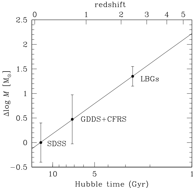
FIG. 14.— The points show the displacement in mass applied to the SDSS M-Z relation (for which \Delta \log M \equiv 0 by definition) to match the GDDS+CFRS and LBG distributions. This describes how much more massive a high- z galaxy with a given metallicity would roughly be with respect to local galaxies with similar metallicities. The error bars indicate the \sim 1\sigma mass dispersion at the median metallicity in the samples, as seen in Figure ???. The small error bar for the LBGs is the effect of the small sample. The straight line is the linear correlation of the three points (Eq. ??).
