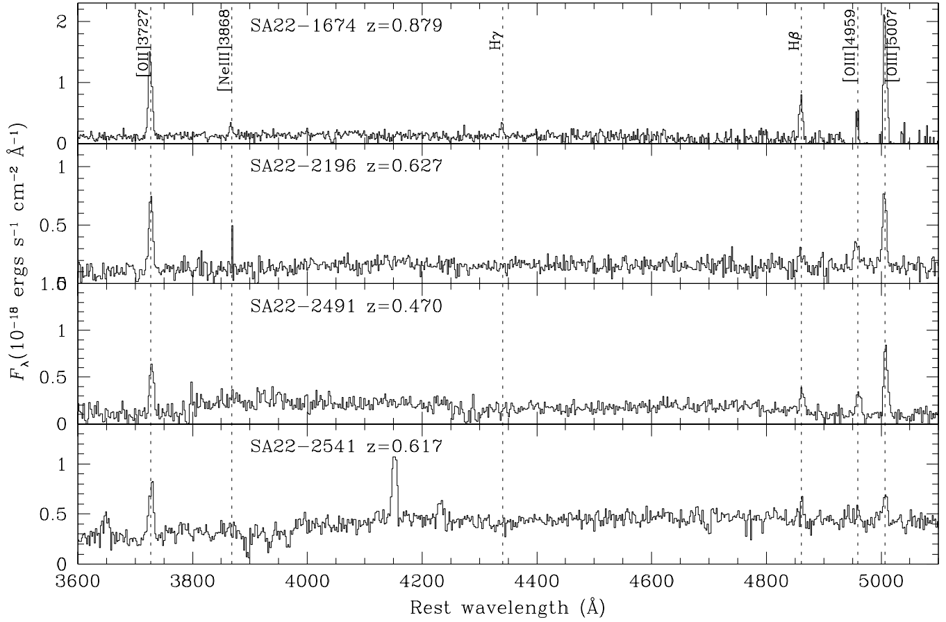
FIG. 5.— As in Figure ???. The two spurious emission lines at \lambda \sim 4200 \text{ \AA} in the spectrum of SA22-2541 are due to order overlap in the GMOS mask (see text).
