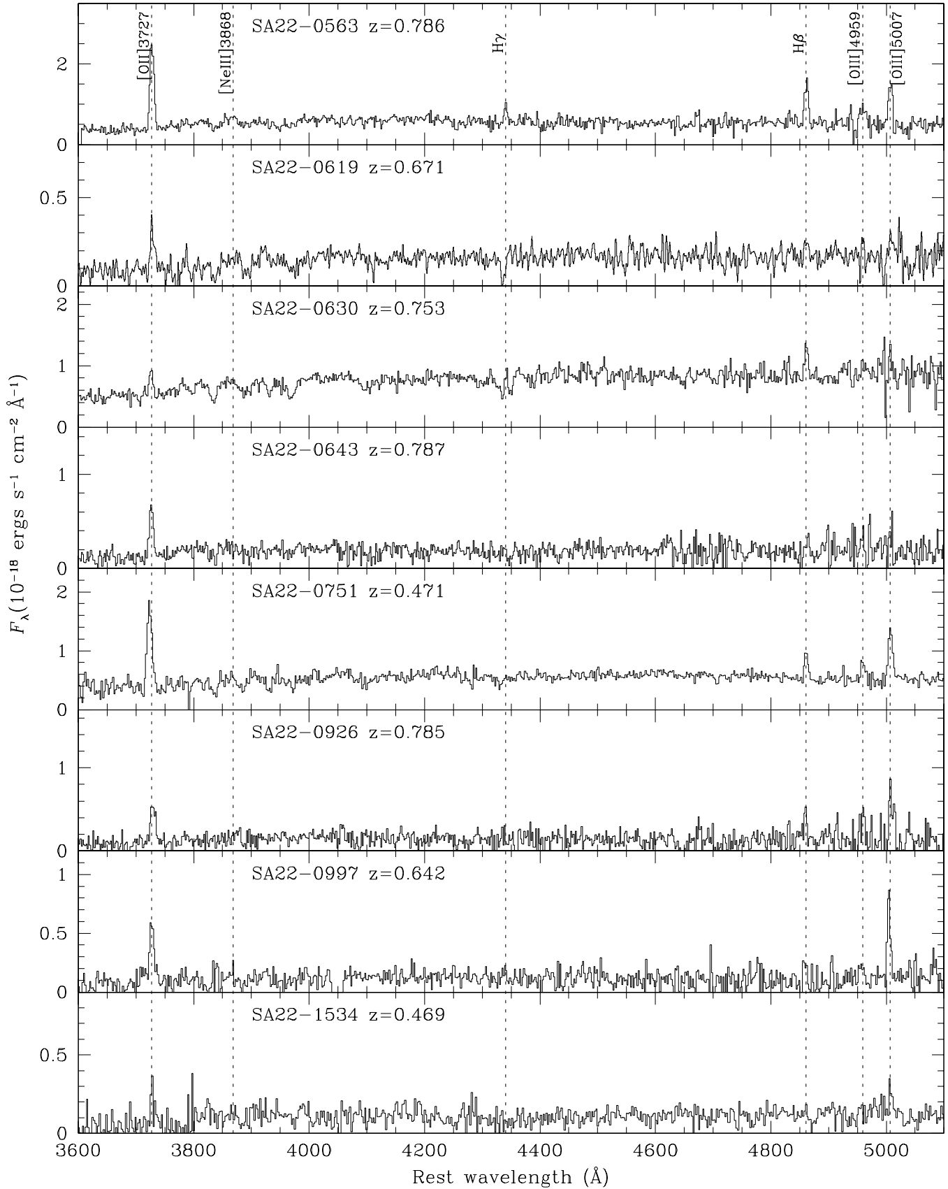
FIG. 4.— As in Figure ??.
