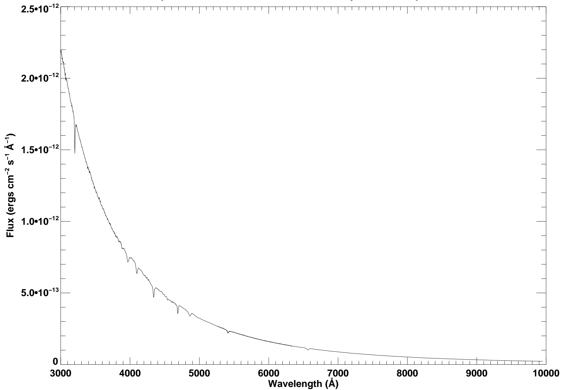
BD+28 4211 absolute spectrum obtained from http://www.stsci.edu/hst/observatory/cdbs/calspec.html
