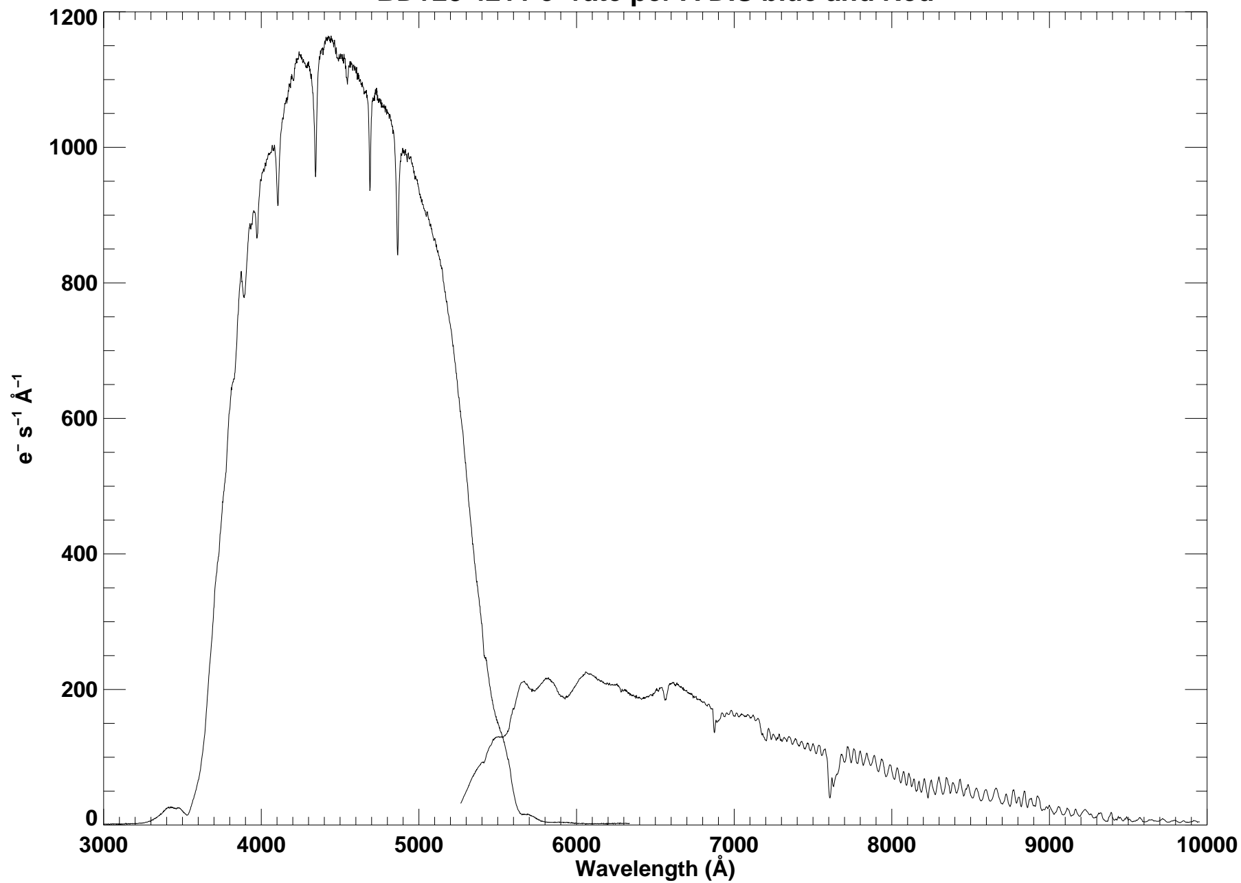
BD+28 4211 e - rate per Å DIS blue and Red
