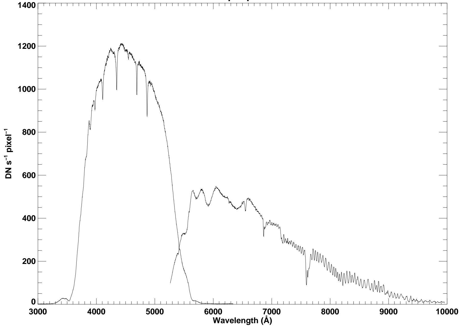
BD+28 4211 DN rate per pixel DIS blue and Red
