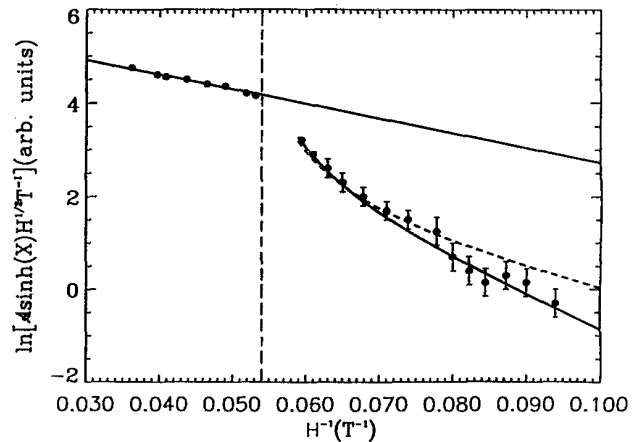
FIG. 1. \ln[\mathcal{A} \sinh(X)H^{1/2}T^{-1}] in V_3Si as a function of 1/H , where X = 2\pi^2 T/\hbar\omega_c and \mathcal{A} = \mathcal{A}^{\mathcal{G}}(H, T) + \mathcal{A}^{1-\mathcal{G}}(H, T) . Full circles represent the experimental data of Corcoran et al. [2]. The dashed line is a theoretical result obtained from Eqs. (7) and (8), with \Gamma set to \Gamma_0 = 0.36 meV, while the full line uses \Gamma evaluated self-consistently (9). The vertical dashed line indicates the normal-superconductor transition at H_{c2} = 18.5 T. We have used \Delta_0 = 2.6 meV and the effective mass of 1.6m_e and 1.7m_e in the normal and vortex states, respectively. (From Ref. [3].)
