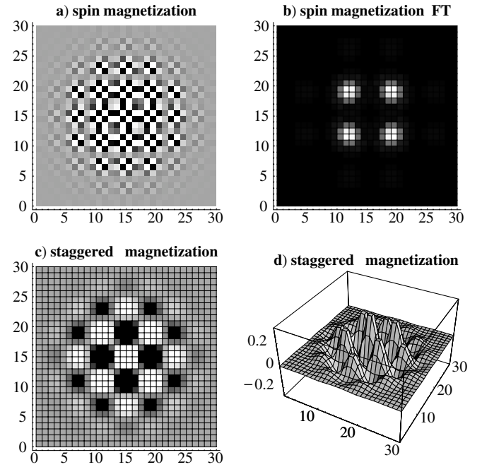
FIG. 1. Magnetization M_i and staggered magnetization M_i^S induced in the vicinity of the fluctuating vortex. Parameters used: t = 1 , \Delta_0 = 0.7 , \mu = -1.6 resulting in maximum gap of 2.3 and average charge density n = 0.62 electrons per site, \mathcal{V}_0 = 1.0 and \ell_v = 12 ; periodic boundary conditions.
