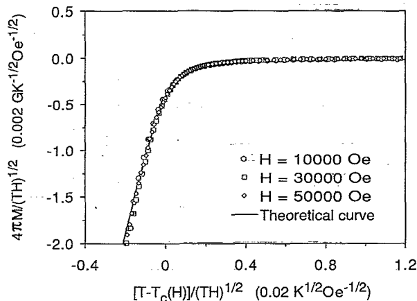
FIG. 1. 2D scaling of magnetization data for \text{Bi}_2\text{Sr}_2\text{Ca}_2\text{Cu}_3\text{O}_{10} in various magnetic fields parallel to the c axis. The theoretical curve is obtained from scaling function f'(x) given by Eq. (7).
